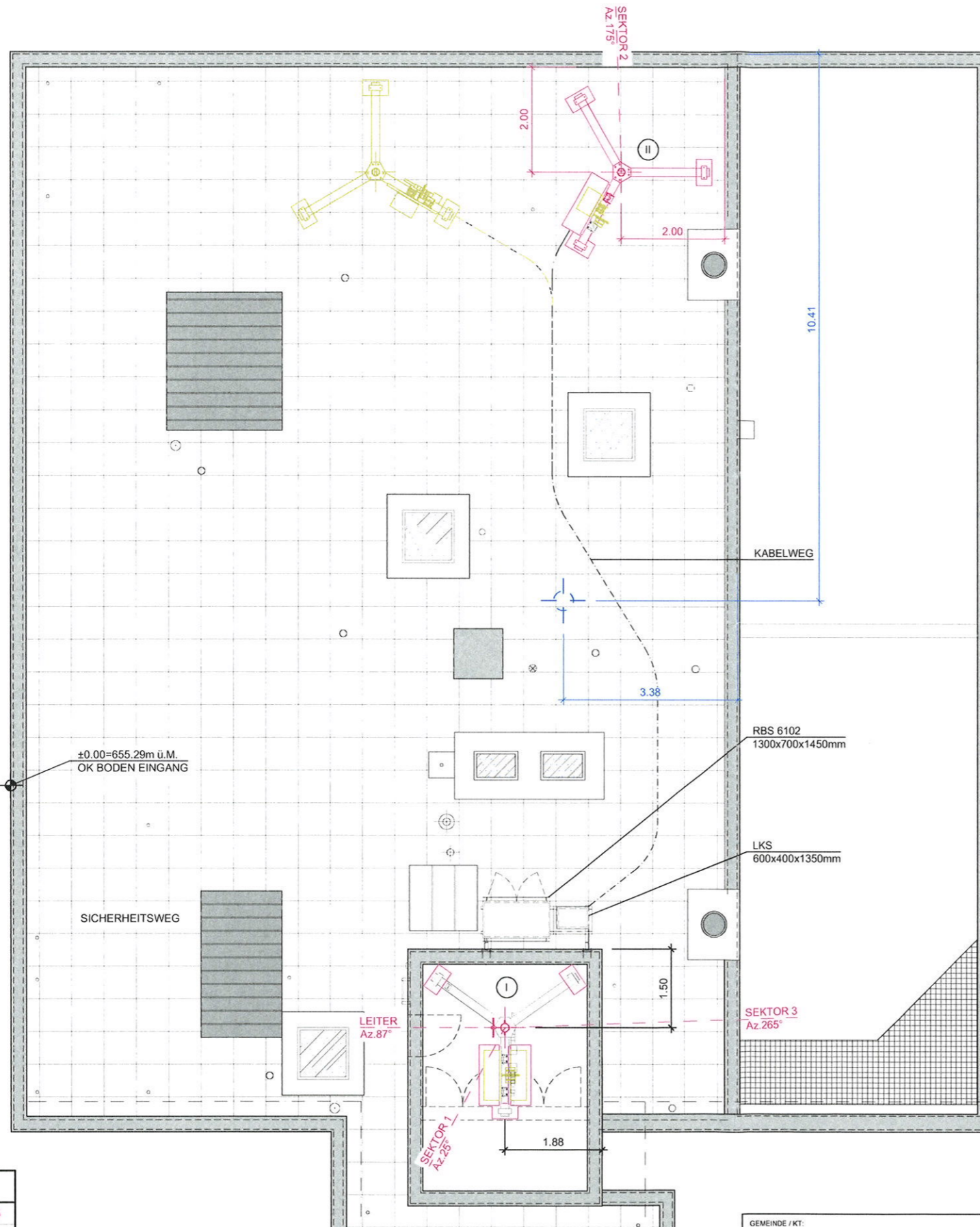
Situation 1:100
